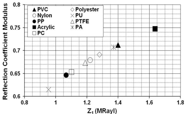
Fig. 4b. Zoom of reflection coefficient simulation at 10 MHz as a function of polymers delay line on glycerin at room temperature (20 °C).
