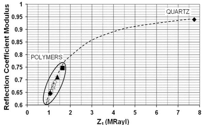
Fig. 4a. Reflection coefficient simulation at 10 MHz as a function of the delay line materials on glycerin at room temperature (20 °C).
