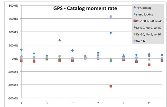
Figure C2. GPS minus catalog moment rate variability. Variations in the median differences between GPS and catalog moment rate in each source zone expressed as a percentage relative to the reference model ((test – reference)/reference). Source zones from 1 to 12 follow the order in Tables 1 and 2.
