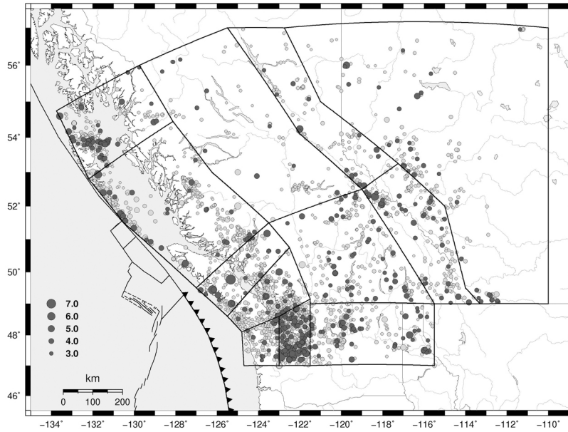
Figure 2. Earthquakes and seismic source zones. Continental crustal earthquakes from GSC catalog, magnitude M \geq 2.0 , 1899–2009 (light gray circles). Dark gray circles show earthquakes M \geq 3.0 that pass completeness test. Earthquakes occurring in the oceanic plates, along the Queen Charlotte and Cascadia plate-boundary faults (Figure 1), and induced earthquakes are omitted.
