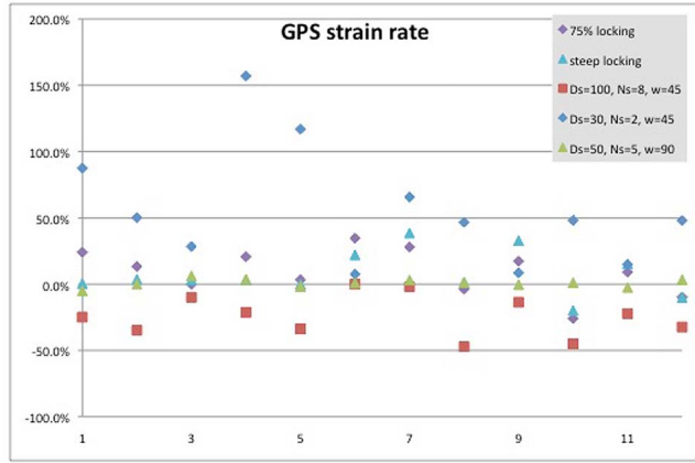
Figure C1. Strain rate variability. Variations in average scalar strain rate in each source zone expressed as a percentage relative to the reference model ((test – reference)/reference). Source zones from 1 to 12 follow the order in Tables 1 and 2.
