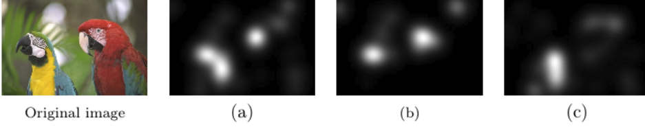
Figure 3. Effects of global weighting. a) heatmap generated with default parameters ( Wc = Wi = Wo = 1.0 ), b) heatmap generated with lower color weights ( Wc = 0.5 ), c) heatmap generated with high color weight ( Wi = Wo = 0.5 ).
