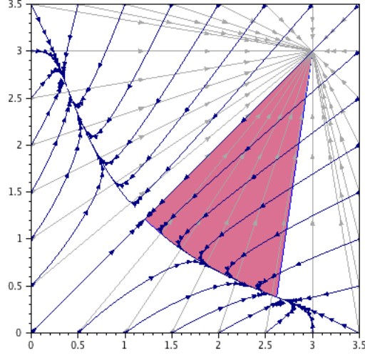
Figure 3: Vector fields F^0 (grey lines) and F^1 (blue lines) of the example in Section 5.4 with \alpha = 3 . The shaded region is \gamma^+(a, a^{-1}) \times E .
