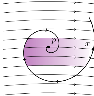
Figure 2: The flows near the attracting point p in Proposition 5.5.
