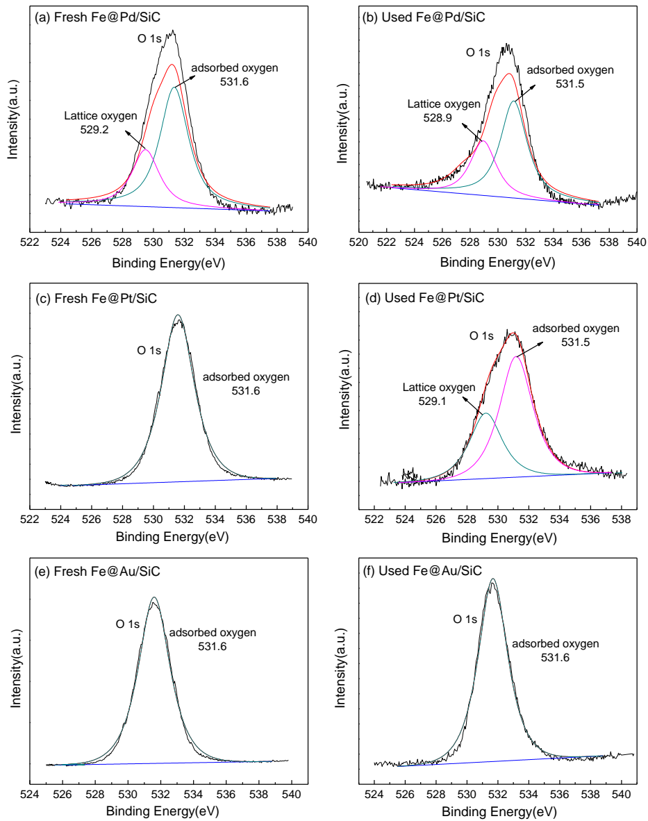
Fig.8 XPS spectra of O 1s levels of fresh and used Fe@Pd/SiC (a and b), Fe@Pt/SiC (c and d) and Fe@Au/SiC (e and f). 25
