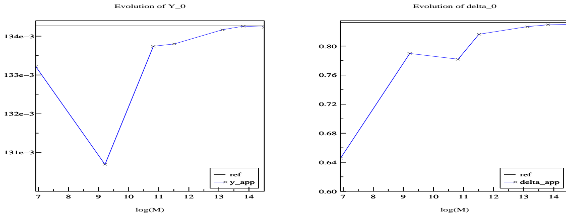
Figure 3: Evolution of \bar{Y}_0^{q,p,N,M} and \delta_0 := \frac{\bar{Z}_0^{q,p,N,M}}{\sigma_{S_0}} w.r.t. \log(M) when N = 20 , p = 2 , q = 5 -Discrete Down and Out Barrier Call option
