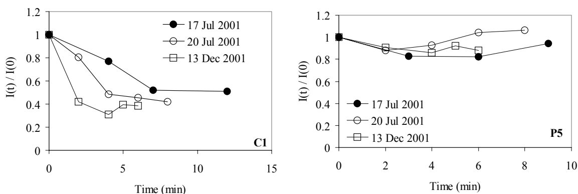
Figure 2. Evolution of the perceived odor intensity in the living room for 2 panelists. Data are normalized by the initial perceived intensity I(0) .
