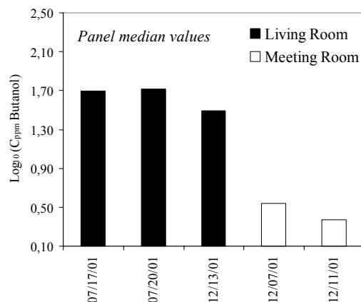
Figure 1. Odor intensity ratings in the living room and in the meeting room upon entering. The Y-scale covers the whole linear scale from the weak (0.1) to the strong reference (2.5).
