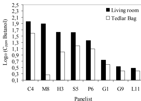
Figure 3. Comparison of the initial odor intensity ratings in the living room with assessments of sampled air in Tedlar ® bags (12/13/01 evaluation).
