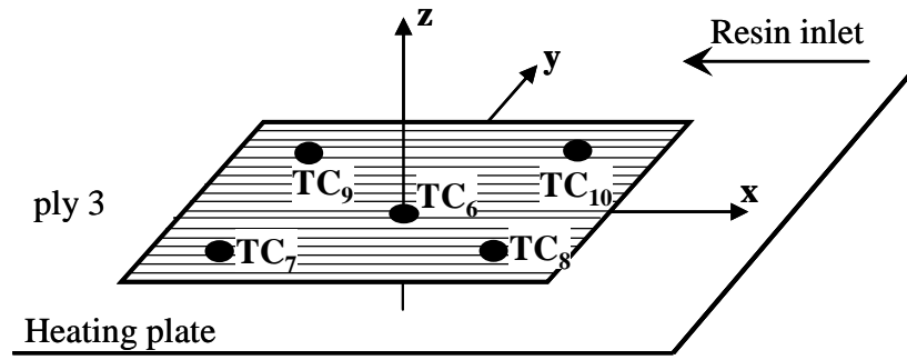
Fig.13 Positions of micro-thermocouples (TC) in the preform stacking in closed lid test of the 2 nd experimental conditions.
