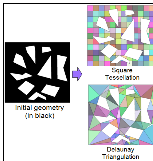
Fig. 2. Example of Tessellations (square and triangle).
