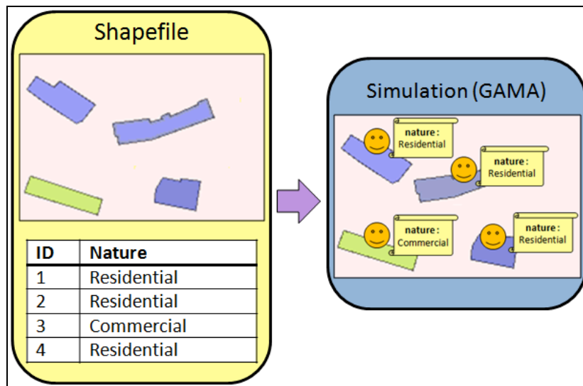
Fig. 1. Example of geographic data agentification
