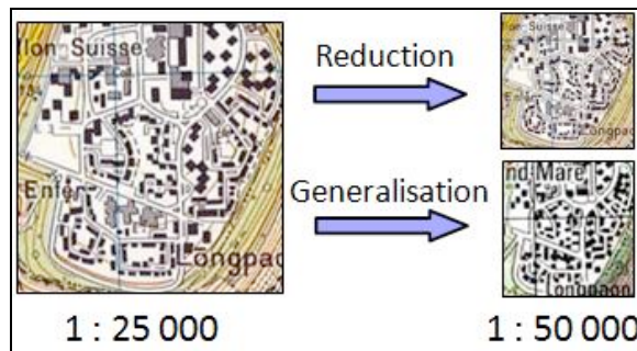
Figure 1. Cartographic Generalisation
