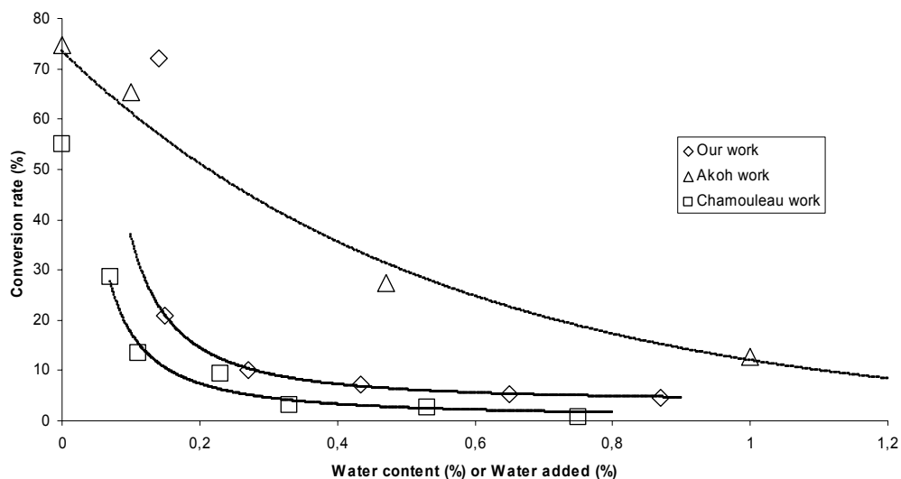
Fig. 1 : Conversion rate as a function of the initial water content (Chamouleau and our works) or water added (Akoh work)
