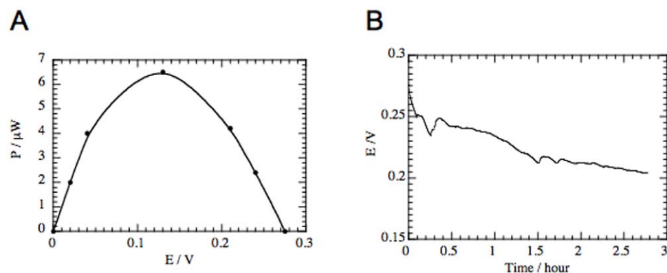
Figure 3. Performance of a “Quinone-Ubiquinone GBFC” implanted in a male Wistar rat (514 g weight). (A) Power-voltage profile. A peak power of 6.5 \mu\text{W} is observed at 0.13 V, yielding a maximum specific power of 24.4 \mu\text{W mL}^{-1} . (B) Discharge curve. Discharge of the GBFC starts 4 hours after implantation. The chronopotentiometry was recorded for a constant current ( 10 \mu\text{A} ). A stable production of more than 2 \mu\text{W} is observed for several hours. doi:10.1371/journal.pone.0010476.g003
