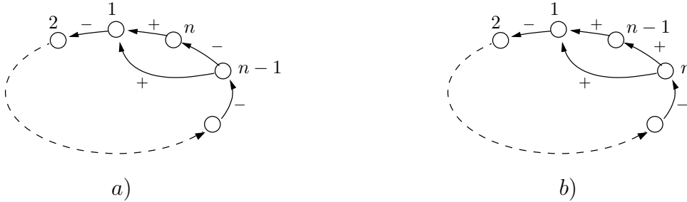
Figure 5: Two networks R_i = (G, F, s_i) , i \in \{1, 2\} whose signed digraphs are différent. The numbers near the vertices indicate the image of the vertices by the update schedule s_i , i \in \{1, 2\} .
