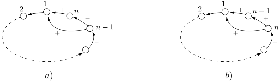
Figure 5: Two networks R_i = (G, F, s_i) , i \in \{1, 2\} whose signed digraphs are différent. The numbers near the vertices indicate the image of the vertices by the update schedule s_i , i \in \{1, 2\} .
