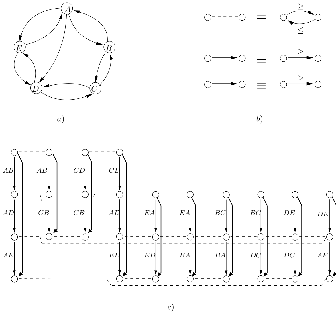
Figure 9: a. A digraph G , instance of \#Cycle\ Cover . b. Caption of figure c. c. Transformation of G into the digraph H , instance of \#OA . Here, we represent \mathcal{RO}(H) . In the intention of keeping the figure simple, we only have labelled the arcs representing an arc of G .
