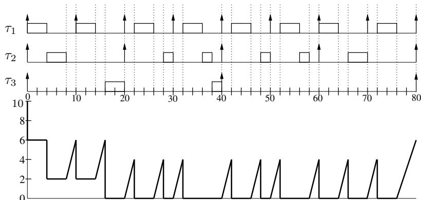
Figure 1: EDF_{asap} : Battery \mathcal{B}(10, 2) and e_1 = e_2 = e_3 = 1
