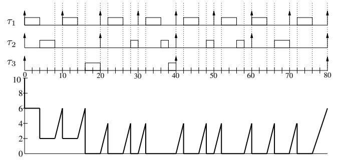
Figure 1. EDF_{asap} : Battery \mathcal{B}(10, 2) and e_1 = e_2 = e_3 = 1
