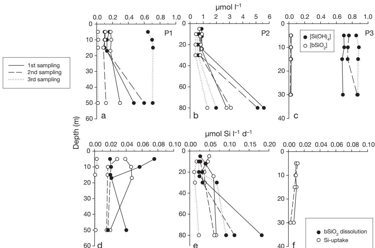
Fig. 4. (a,b,c) Vertical distribution of Si(OH)_4 and bSiO_2 ( \mu mol\ l^{-1} ) and (d,e,f) bSiO_2 production and dissolution ( \mu mol\ Si\ l^{-1}\ d^{-1} ) in the euphotic layer (100–50 to 25–1% photosynthetically active radiation). Process 1 (P1, western SAZ) is shown in Panels a and d, Process 2 (P2, PFZ) is shown in Panels b and e, and Process 3 (P3, eastern SAZ) is shown in Panels c and f. PFZ: Polar Frontal Zone; SAZ: Subantarctic Zone
