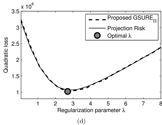
Figure 2: Illustration of the selection of \lambda by minimizing \text{GSURE}_{\Pi} in a compressed sensing problem ( Q/N = 0.5 ) by an \ell^1 -analysis regularization in a shift-invariant Haar wavelet dictionary. (a) The MLE x_{\text{ML}} . (b) A solution x_{\lambda}^*(y) of (\mathcal{P}_{\lambda}(y)) at the optimal \lambda (the one minimizing \text{GSURE}_{\Pi} ). (c) The underlying true image x_0 . (d) Projection risk \text{Risk}_{\Pi} and its \text{GSURE}_{\Pi} estimate obtained from (10) using k = 1 random realization.
