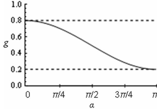
Figure 3. Variation of the gain with the angle \alpha for partially polarized incident light, when p_d and \bar{\tau} are equal to 1. The dashed lines represent the extreme values of the gain p_i = 0.6, \tau_M = 1, \tau_m = 0
