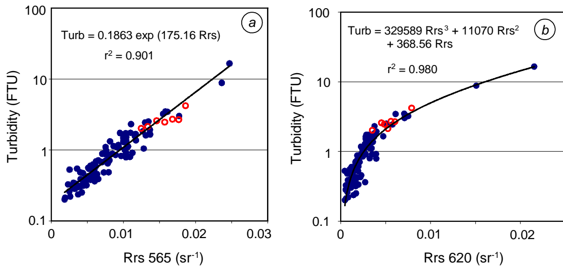
Figure 3. Best-fit two-band algorithm for turbidity in New Caledonia (N=113). 7 stations at the head of bays are distinguished with empty red marks.
