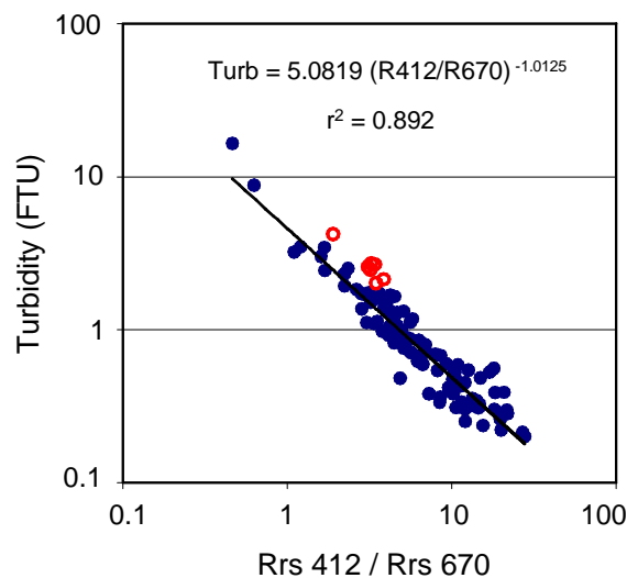
Figure 3. Best-fit two-band algorithm for turbidity in New Caledonia (N=113). 7 stations at the head of bays are distinguished with empty red marks.
