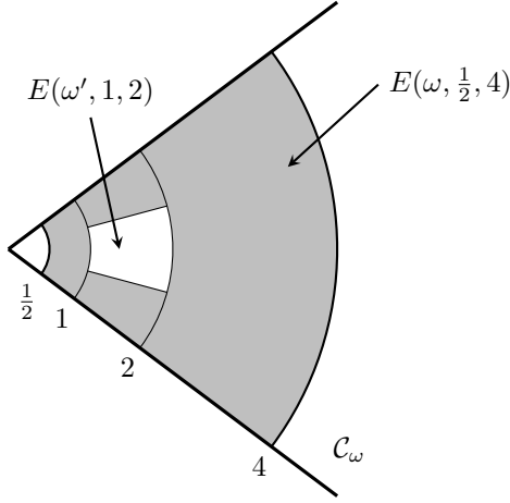
FIGURE 1. The function u in Lemma 2.4 is a supersolution in the grey region \Omega and positive in the white region illustrated above.
