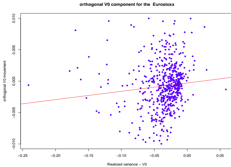
Figure 11: Effect of Realized Volatility on V_0 dynamics for the EUROSTOXX.
