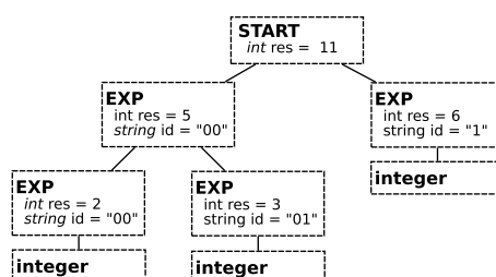
Fig. 1 Example of an attribute grammar which defines a language to add integers. The attributes res are synthesized, id are inherited. The result of the evaluation of programs is the value START.res . id attributes are only shown to illustrate inherited attributes behavior.
