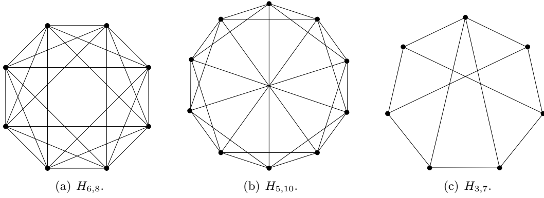
Figure 1: Three examples of Harary graphs.
