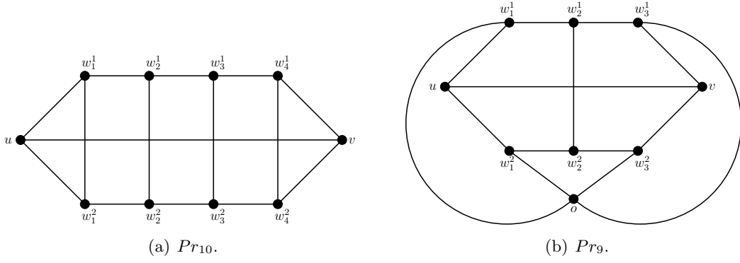
Figure 2: Two examples of Pr graphs.
