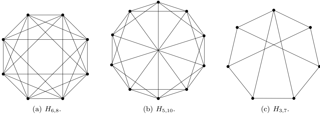
Figure 1: Three samples Harary graphs.
