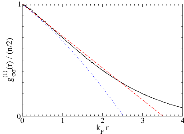
FIG. 4: (Color online) One-body density matrix g_{\sigma\sigma}^{(1)}(r) = \langle \hat{\psi}_\sigma^\dagger(\mathbf{r}) \hat{\psi}_\sigma(\mathbf{0}) \rangle of the homogeneous non-polarized unitary gas at zero temperature: comparison between the fixed-node Monte Carlo results from Ref. [106] (black solid line) and the analytic expression (180) for the small- k_F r expansion of g_{\sigma\sigma}^{(1)} up to first order (red dashed straight line) and second order (blue dotted parabola) where we took the value \zeta = 0.95 extracted from the Monte Carlo data for g_{\uparrow\downarrow}^{(2)} , see Fig. 3.
