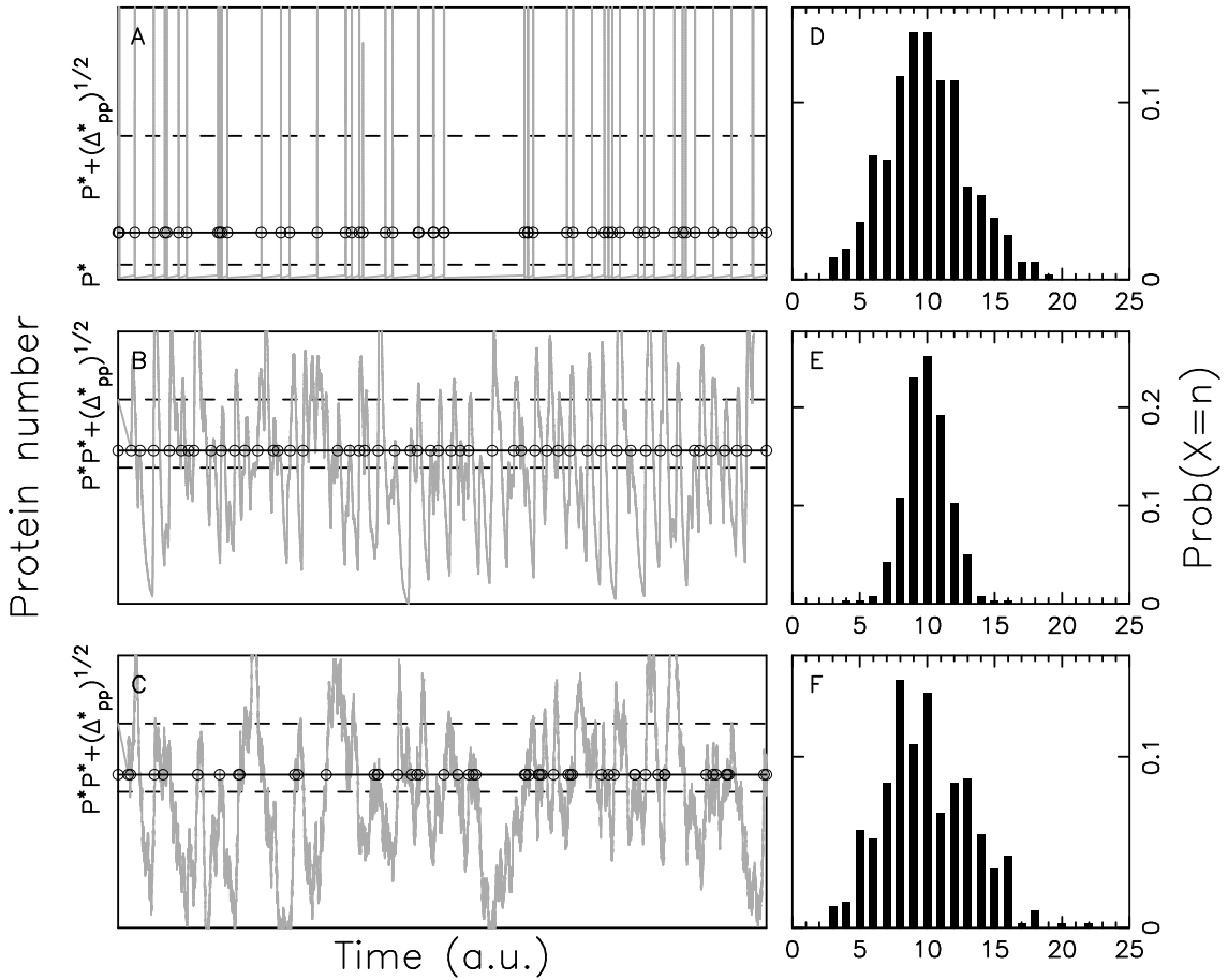
Figure 4: Protein spike antibunching. (A,B,C). Time evolution of protein copy number for \Lambda = 100 , \delta = 1 and \rho = 10^{-3} , 1 , 10^3 , respectively. Dashed lines indicate mean protein level and mean protein level plus standard deviation. Black lines correspond to the high trigger level and spiking events are indicated by black circles. (D, E, F) Probabilities of observing n spikes during a time window of 10 average transition times \rho = 10^{-3} , 1 , 10^3 , respectively.
