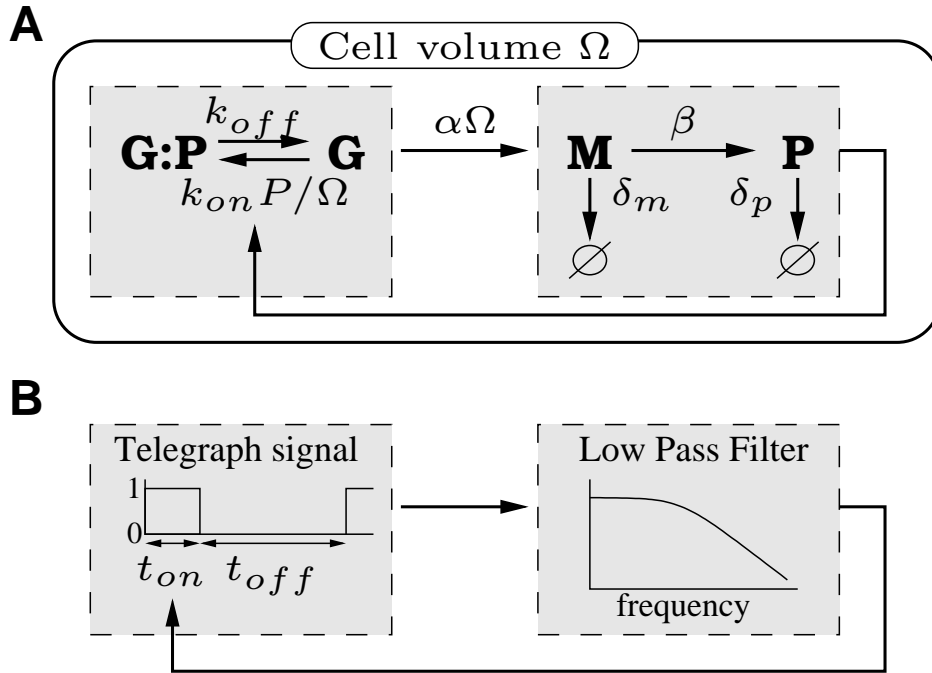
Figure 1: Schematic view of the self-repressing gene network. (A) Biochemical reactions composing the network. P , M , G , and G : P denote protein, mRNA, free gene and bound gene chemical species, respectively. The kinetic constants of the reactions are indicated, with \Omega denoting cell volume. In the limit where \Omega is large, the mRNA and protein copy numbers become macroscopic variables, with decreasing fluctuations, while the gene state remains microscopic and displays full-scale variations. (B) Block diagram representation of the network, consisting of a random telegraph signal generator representing the gene state-flip dynamics, and of a low-pass filter of cut-off frequency \omega_c representing proteins and mRNA dynamics. The telegraph signal regulates its frequency and duty cycle through feedback from the low pass filter.
