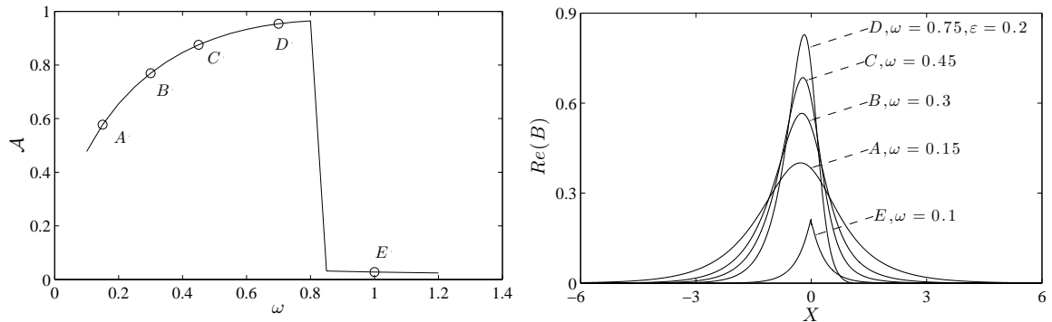
FIGURE 2. cDZ equation: (left) Action \mathcal{A} of ground states as function of the frequency \omega and (right) bifurcation of a peakon from smooth ground states ( \varepsilon = 0.2 ).
