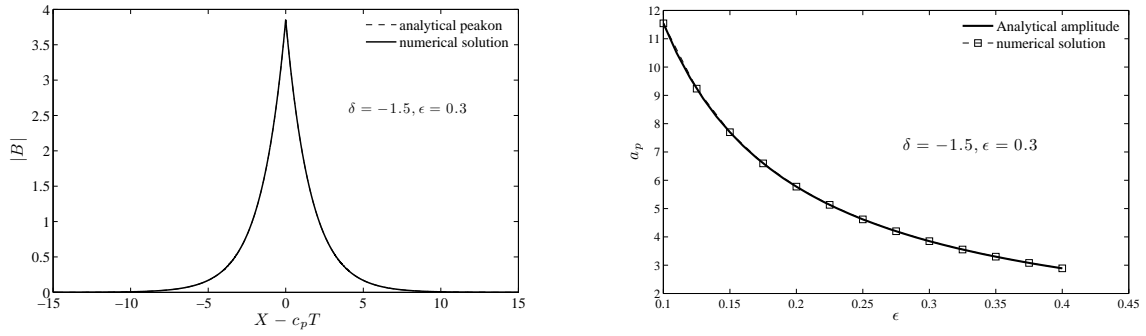
FIGURE 9. Left: numerical peakon (solid) of the perturbed local cDZ equation (2.12) and associated analytical solution (2.13) (dash) for \epsilon = 0.30 , \delta = -1.5 ; Right: amplitude of the numerical peakon against its theoretical counterpart (2.15) as function of \epsilon .
