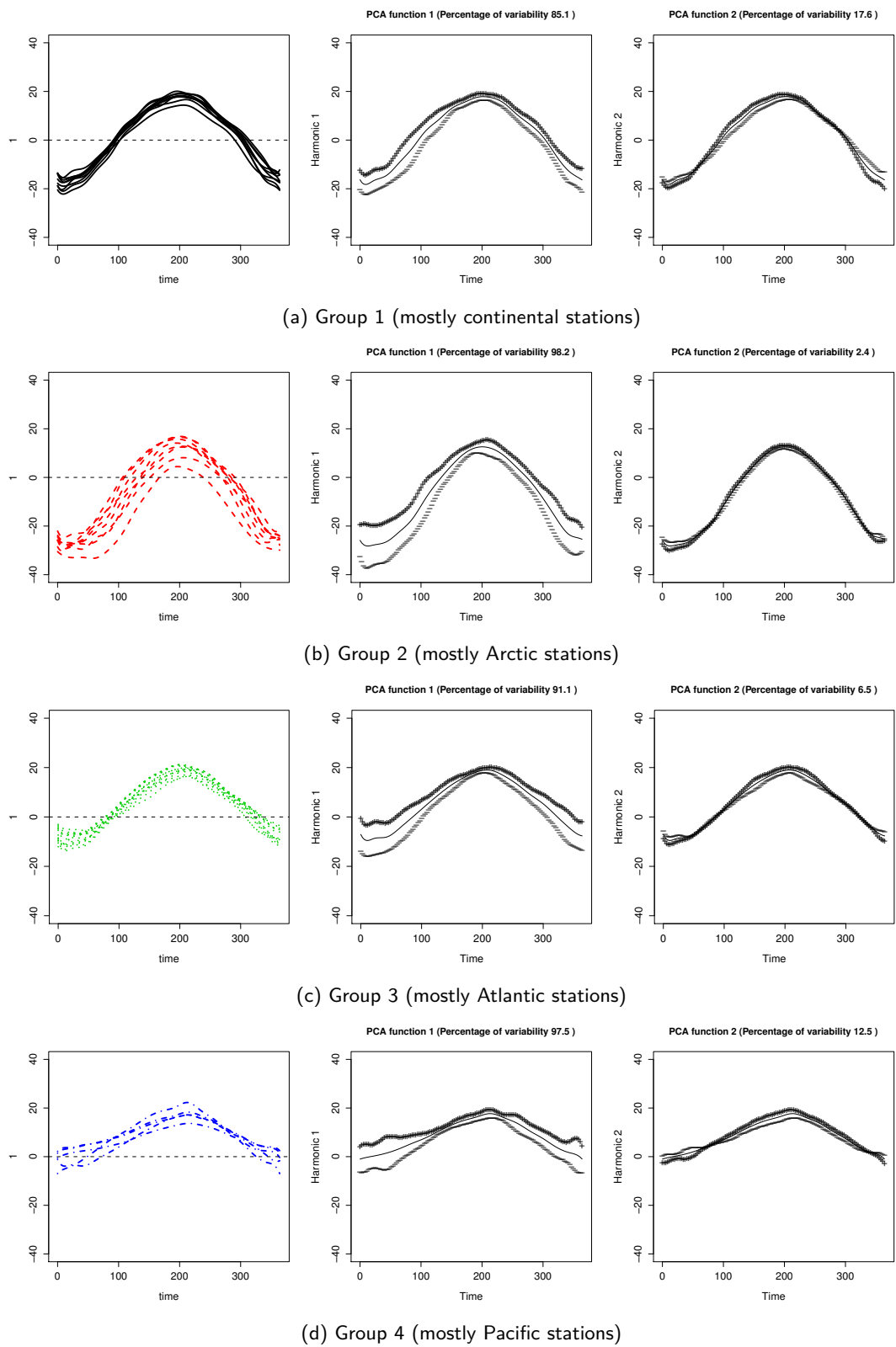
Figure 6: The group means of the Canadian temperature data obtained with pgpEM (left panel) and the effect of adding (+) or subtracting (−) twice the square root of the variance to the cluster means along the two first eigenfunctions (center and right panels, see text for details).
