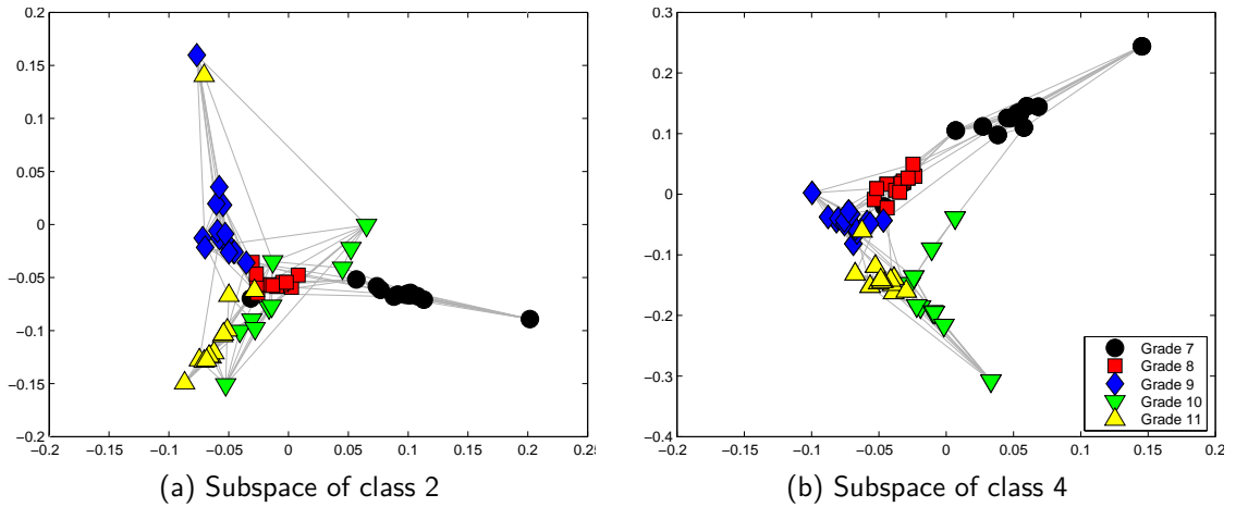
Figure 7: Visualisation of the Add Health network with pgpDA in the feature subspace of the 2nd and the 4th class (grade 8 and 10 respectively).
