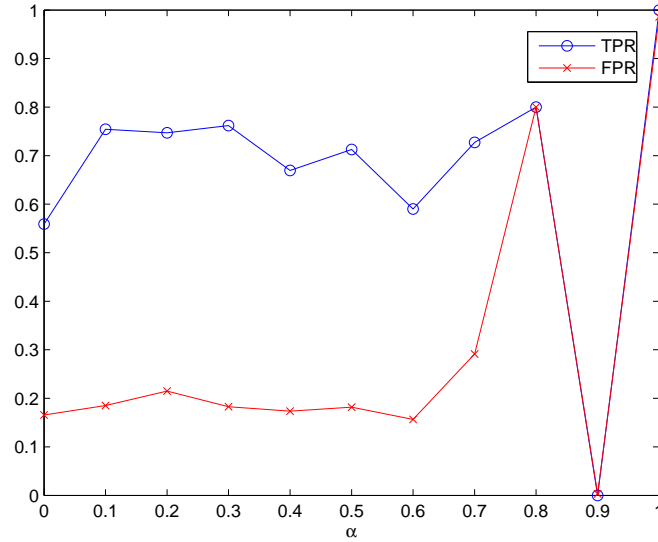
Figure 11: Choice of the mixing parameter \alpha through cross-validation based on true positive rate (TPR) and false positive rate (FPR) curves.
