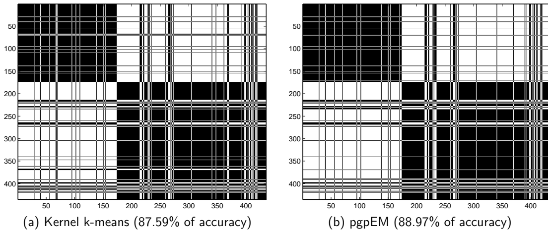
Figure 9: Clustering results of the house-vote dataset obtained with kernel k-means (left) and pgpEM (right). The clustering results are presented through a binary matrix where a black pixel indicates a common membership between two senators. Again, the first 168 congressmen are republicans whereas the 267 last ones are democrats. On this run, pgpEM correctly classifies 6 congressmen more than kernel k-means.
