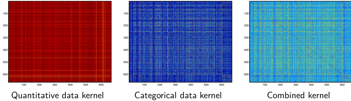
Figure 8: Quantitative (left) and categorical (center) data kernels and the combined kernel (right) for the Thyroid dataset (mixed data).
