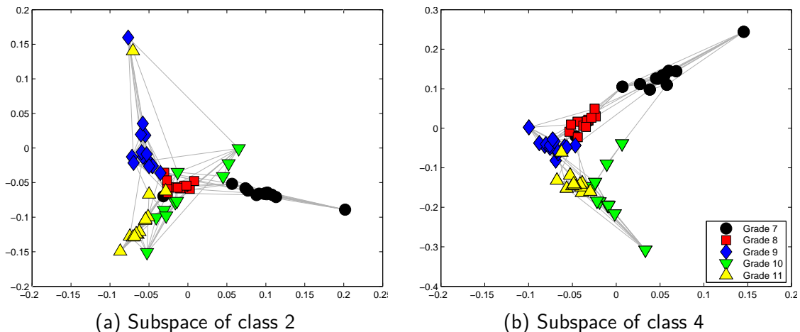
Figure 4: Visualisation of the Add Health network with pgpDA in the feature subspace of the 2nd and the 4th class (grade 8 and 10 respectively).
