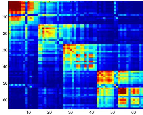
Figure 3: Regularized Laplacian kernel associated to the Add Health network for \nu = 4 : blue pixels correspond to low values (low similarity between nodes) and red pixels correspond to high values (high similarity between nodes).
