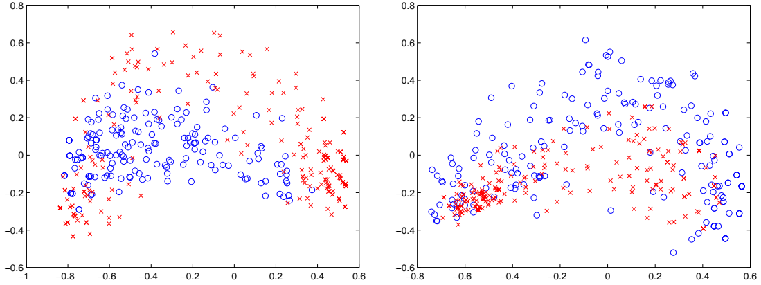
Figure 7: Visualization of the house-vote data in the feature subspace of the republican (left) and the democrat (right) groups (red crosses denote republicans and blue circles denote democrats).
