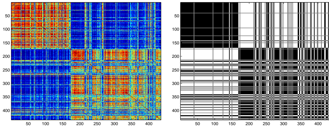
Figure 6: Kernel based on the Hamming distance (left) computed on the house-vote dataset and clustering results (right) obtained with pgpEM. For the kernel, blue and red pixels correspond respectively to low and high values. The clustering results are presented through a binary matrix where a black pixel indicates a common membership between two senators.
