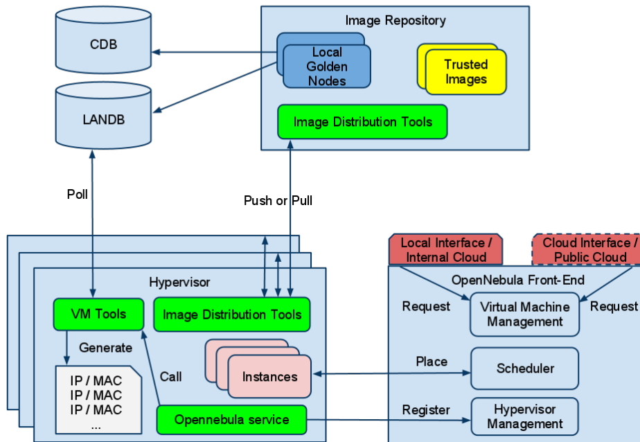
Figure 6.1: High level architecture of Ixcloud
