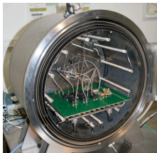
Figure 5: Experimental setup for high-temp characterization
