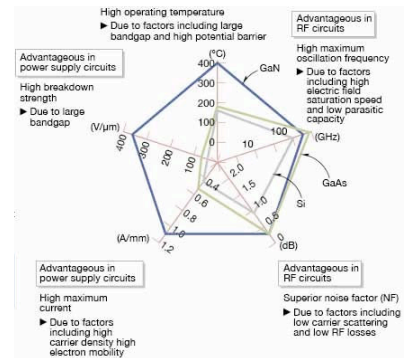
Figure 9: Spider graph of WBG device performances [YOLE 2010]
