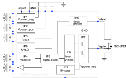
Figure 13: Schematic of a SOI driver [55]
