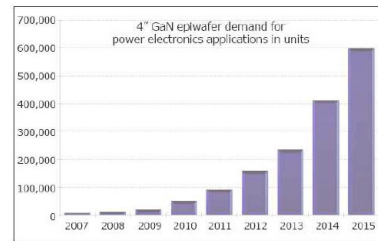
Figure 10: Unit forecast for 4in GaN epiwafers [YOLE 2010]
