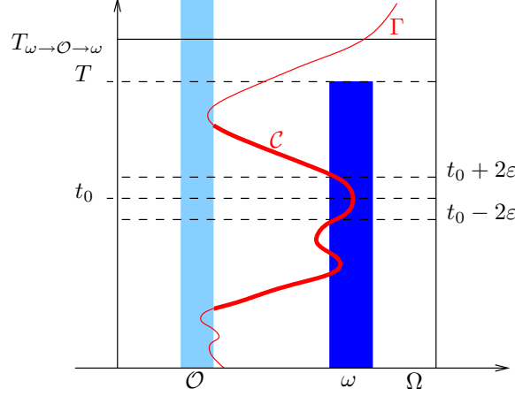
Figure 2: Geometrical situation in the case T < T_{\omega \rightarrow \mathcal{O} \rightarrow \omega} with \pi(\Gamma) \cap ((0, T) \times \omega) \neq \emptyset .
