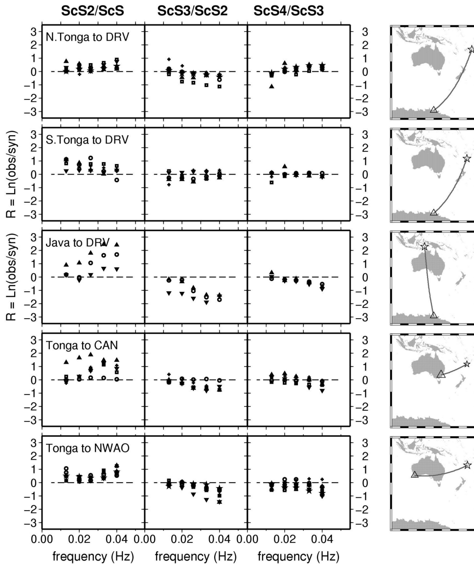
Figure 5. A logarithmic scale representation of the relative ratios (ScS_{n+1}/ScS_n)_{obs}/(ScS_{n+1}/ScS_n)_{syn} as defined in eq. (2), for a selection of paths. Paths are mapped on the right with a triangle representing the station and a star representing the epicentres. For each path, the different symbols in the relative ratio plots correspond to different events. ScS_5/ScS_4 is not shown. The horizontal dashed line corresponds to PREM. The linear trends in relative ratios indicate that Q is globally independent of frequency. A positive (respectively negative) slope corresponds to a Q -value larger (respectively smaller) than the PREM one. Note the coherence of results for the different events corresponding to a same path, and the variations of slopes between paths and between different multiple ScS_n waves.
