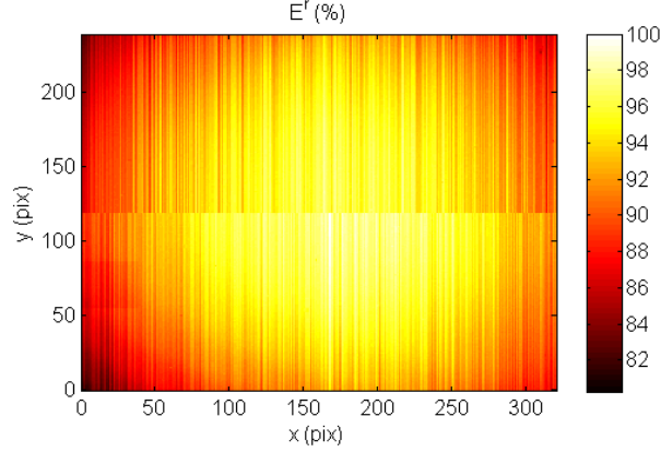
Figure 2. Non-corrected image of the black body, normalized by the maximum value of the image (50 mm prime lens, black body temperature = 25 °C, IT = 1400 \mu s). The “unmatched columns” and the step between the upper and lower halves are electronic artefacts, corresponding to 4-channels multiplexed ROC.
