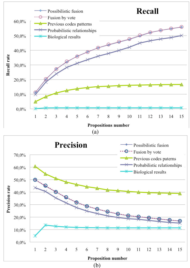
Fig. 2: Evaluation results of the recall (a) and precision (b) rates.
