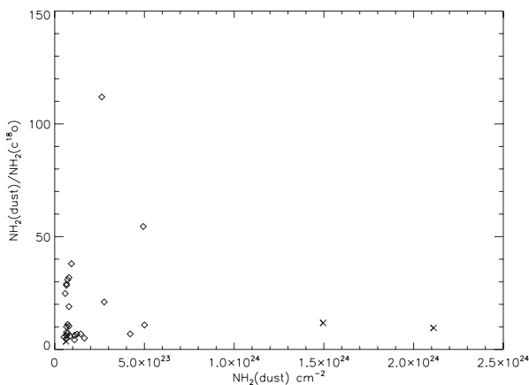
Figure 8. Orion NGC 2024 using CO-derived temperatures to estimate F_{\text{dep}} (left) and using dust temperatures (right). Squares represent starless cores and crosses protostellar cores.
