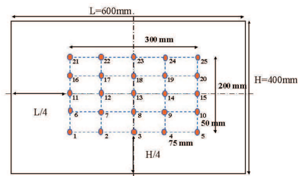
Figure 2: Position of the 25 measure points in plate P_1 and in the corresponding 25 points in plate P_2
