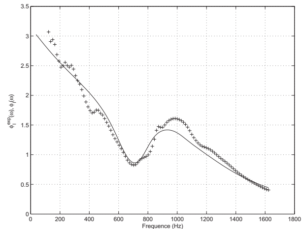
Figure 8: Graphs of \phi_I(\omega) (solid line) and \phi_I^{exp}(\omega) (cross) over the frequency band [100,1600] Hz
