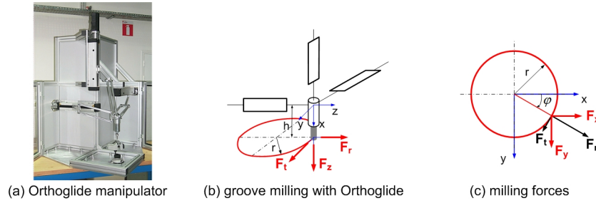
Fig. 3 Milling forces and trajectory location for groove milling using Orthoglide manipulator.
