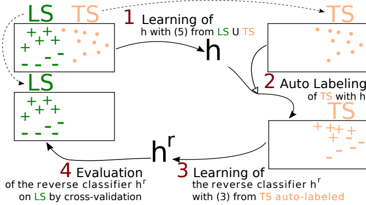
Fig. 4. The reverse validation process in the \phi^R -space. Step 1: Learn the classifier h with the Problem ( DASF_{opt} ). Step 2: Auto-label the target sample with h . Step 3: Learn the reverse classifier h^r on the auto-labeled target sample with the Problem ( SF_{opt} ). Step 4: Evaluate h^r on the source sample (with a k -folds process).
