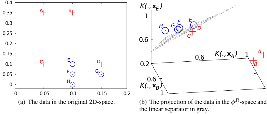
Fig. 3. A set of positive (red crosses) and negative (blue circles) points.
