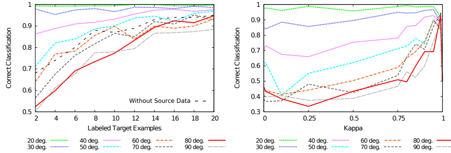
(a) The average rates for each rotation angle according to the quantity of labeled target examples in the learning sample. The result obtained without source data ( i.e. considering only target labels) is indicated with the dashed black line with big dashes. (b) The average rates according to \kappa with 10 target labeled examples, \lambda=0.15 and \beta=0.75 .
