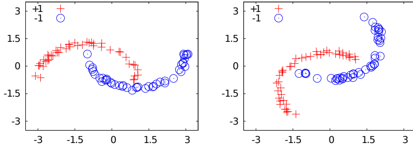
Fig. 6. Toy Problem: On the left: a source sample. On the right: a target sample with a 50^\circ rotation.
