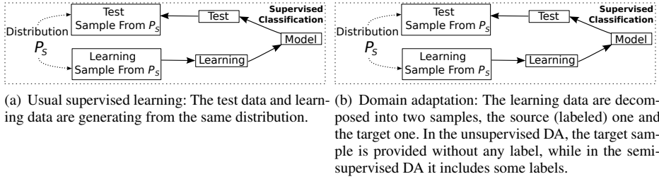
Fig. 1. The intuition behind the difference between a classical machine learning setting and a classical domain adaptation setting. P_S is the distribution generating the source data, P_T is the distribution generating the target data. Note that to simplify the presentation, we use an abuse of notation for distributions generating the samples: unlabeled data of the test and target samples are not exactly drawn from the same distribution used to generate the labeled learning data, see Section 2 for a more formal description.
