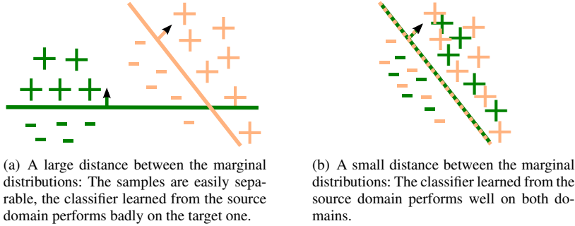
Fig. 2. The intuition behind Theorem 1. The source domain points are in (dark) green (pos.+ , neg.-), the target domain points are in (light) orange.
