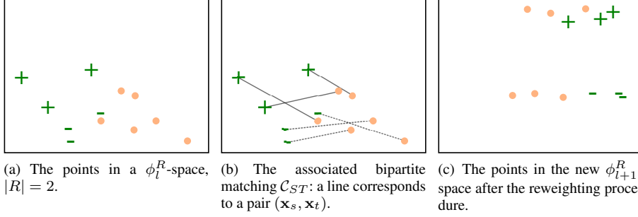
Fig. 5. An iteration of DASF. The source points are in (dark) green (pos. +, neg. -), the unlabeled target ones are (light) orange circles.
