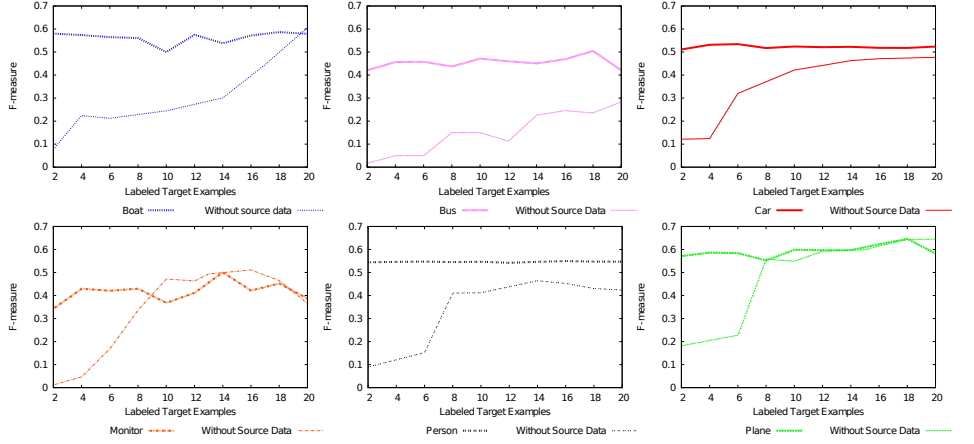
(a) The F-measure according to the quantity of labeled target examples in the learning sample. “Without Source Data” corresponds to the result obtain with a SF-classifier learned only from the target labeled sample.
