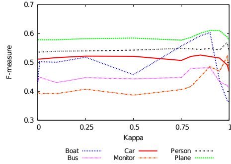
(b) The F-measure according to \kappa with 10 labeled target examples, \lambda = 0.15 and \beta fixed.
