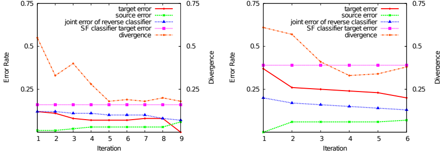
Fig. 8. Toy Problem: Two DASF runs. On the left for a 30^\circ rotation, on the right for a 50^\circ rotation. On the left y -axis is the error rate, on the right y -axis is the divergence measure. We provide the error rates of the classifiers h_t built at each iteration on the source and target test samples, the divergence \hat{d}_{\mathcal{H}\Delta\mathcal{H}} , the reverse classifier joint error, the error on the target test sample of a SF-classifier learning without DA as a baseline.
