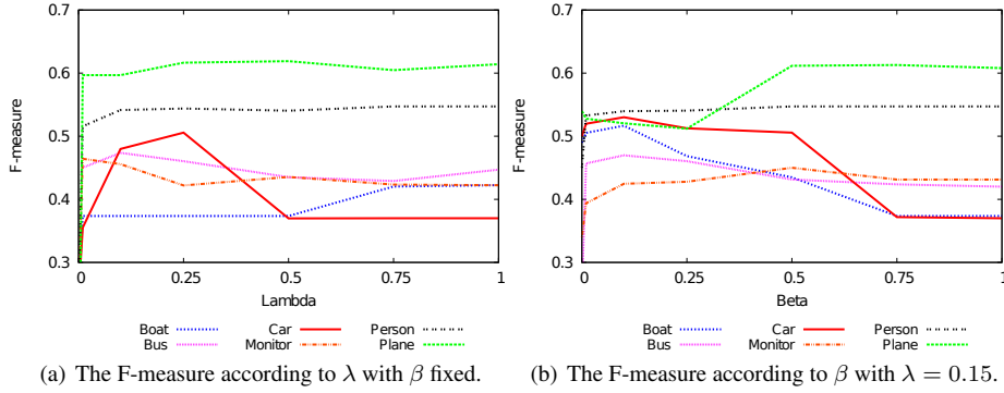
Fig. 13. Image Classification: The results for each concept according to \lambda and \beta in Problem ( DASF_{opt} ), with DASF.
