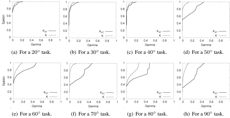
Fig. 7. Toy Problem: Goodness of the similarities over the target samples: \epsilon (Epsilon), as a function of \gamma (Gamma).
