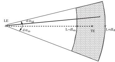
Figure 3. Description of the tolerance parameters. Chord of the nominal profile (dashed line) - Chord of the manufactured profile (solid line) - Localisation of the trailing edge (TE) (gray zone).
