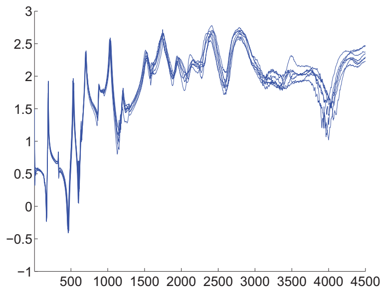
Figure 3: Graphs of the 8 experimental cross FRF between point N_0 and point N_2 corresponding to the 8 sandwich panels. Horizontal axis: frequency in Hertz. Vertical axis: \log_{10} of the modulus of the acceleration in m/s^2 .
