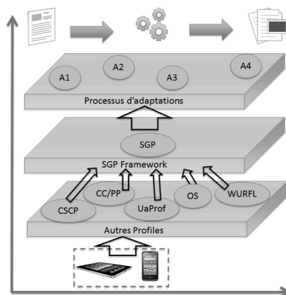
Figure 12. Framework SGP
