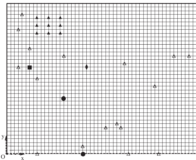
Figure 1. Finite element mesh of the dynamical system: attached spring (■), attached lumped mass (●), attached set of 3 single DOF linear oscillators (Δ), vibration absorbers (▲), excitation node (◆), simply supported boundary (thick line), free boundary (thick dashed line).
