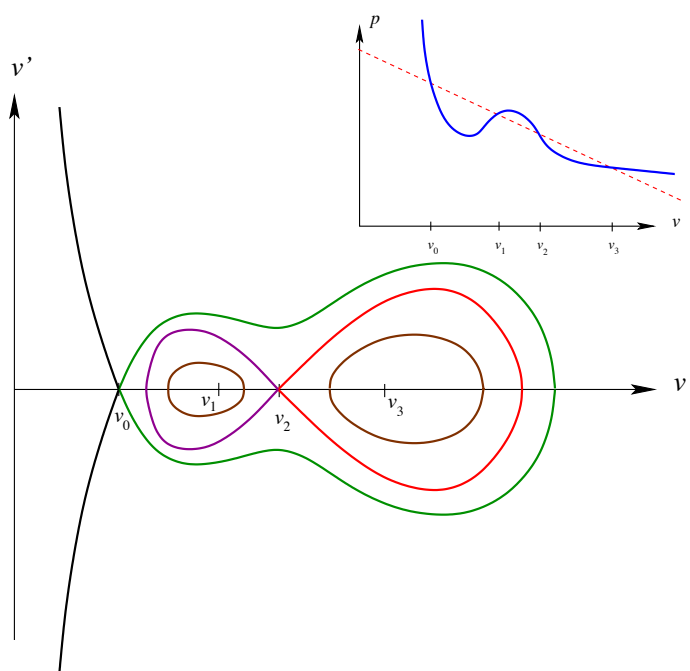
Figure 4: A nonconvex pressure law and the associated phase portrait for capillary profiles. (Observe that equal area rule yields three solitons.)
