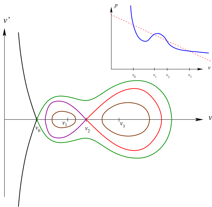
Figure 4: A nonconvex pressure law and the associated phase portrait for capillary profiles. (Observe that equal area rule yields three solitons.)
