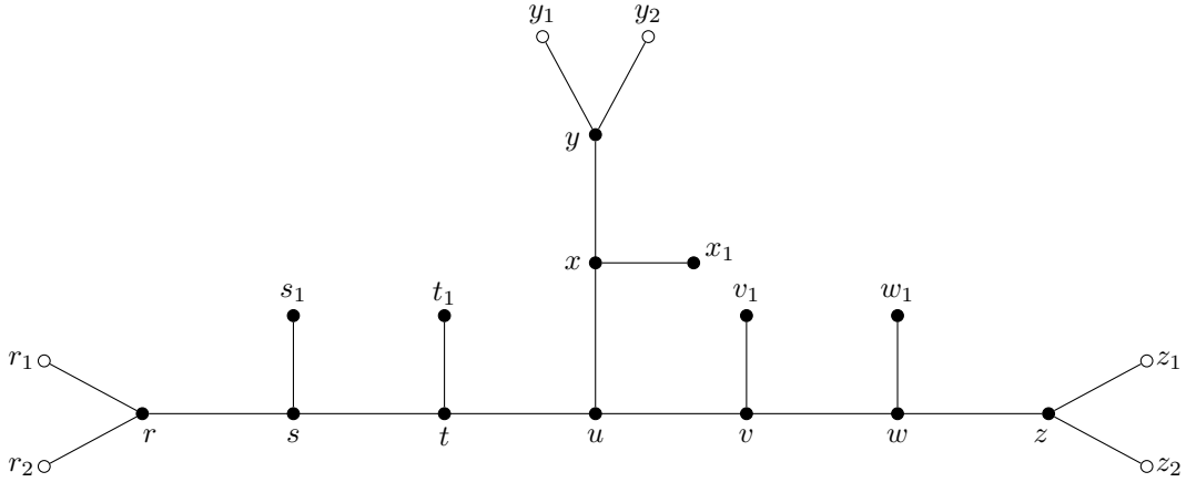
Figure 2: The configuration of Claim 2.6
