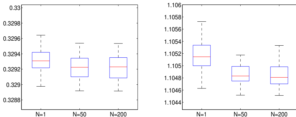
Figure 1: Boxplots of quantization error for n = 10 obtained after 100 runs: N(0, I_2) (left) and N(0, \Sigma_2) (right).
